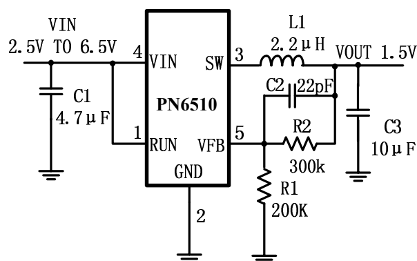
Figure 1. Basic Application Circuit with PN6510 adjustable version
